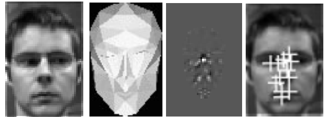
Figure 3: From left: The lowpass filtered incoming video, the weighting (the cosine of the angle between the surface normal and the camera direction), the final rating and the extracted feature points.
